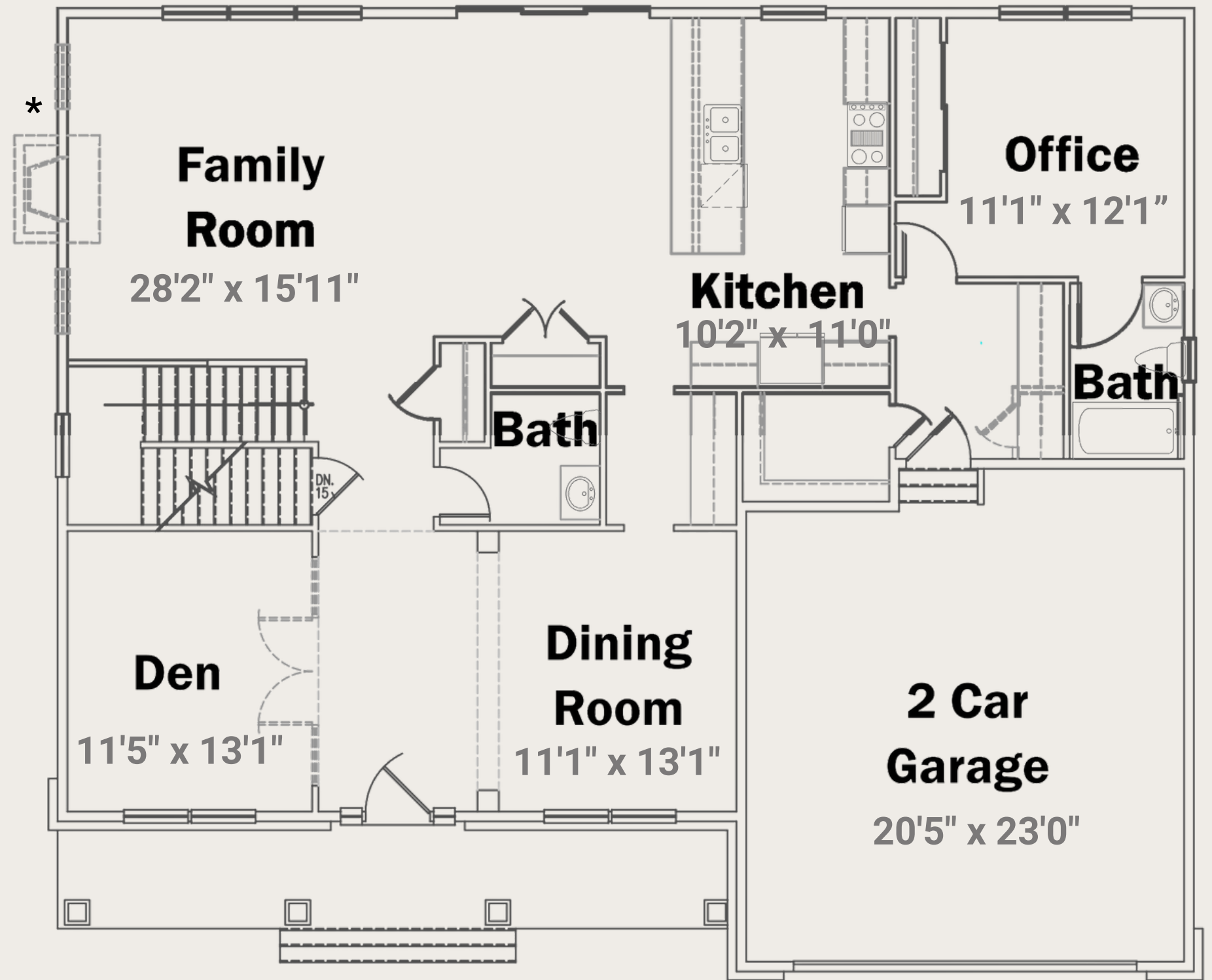
First Floor The Hallmark
