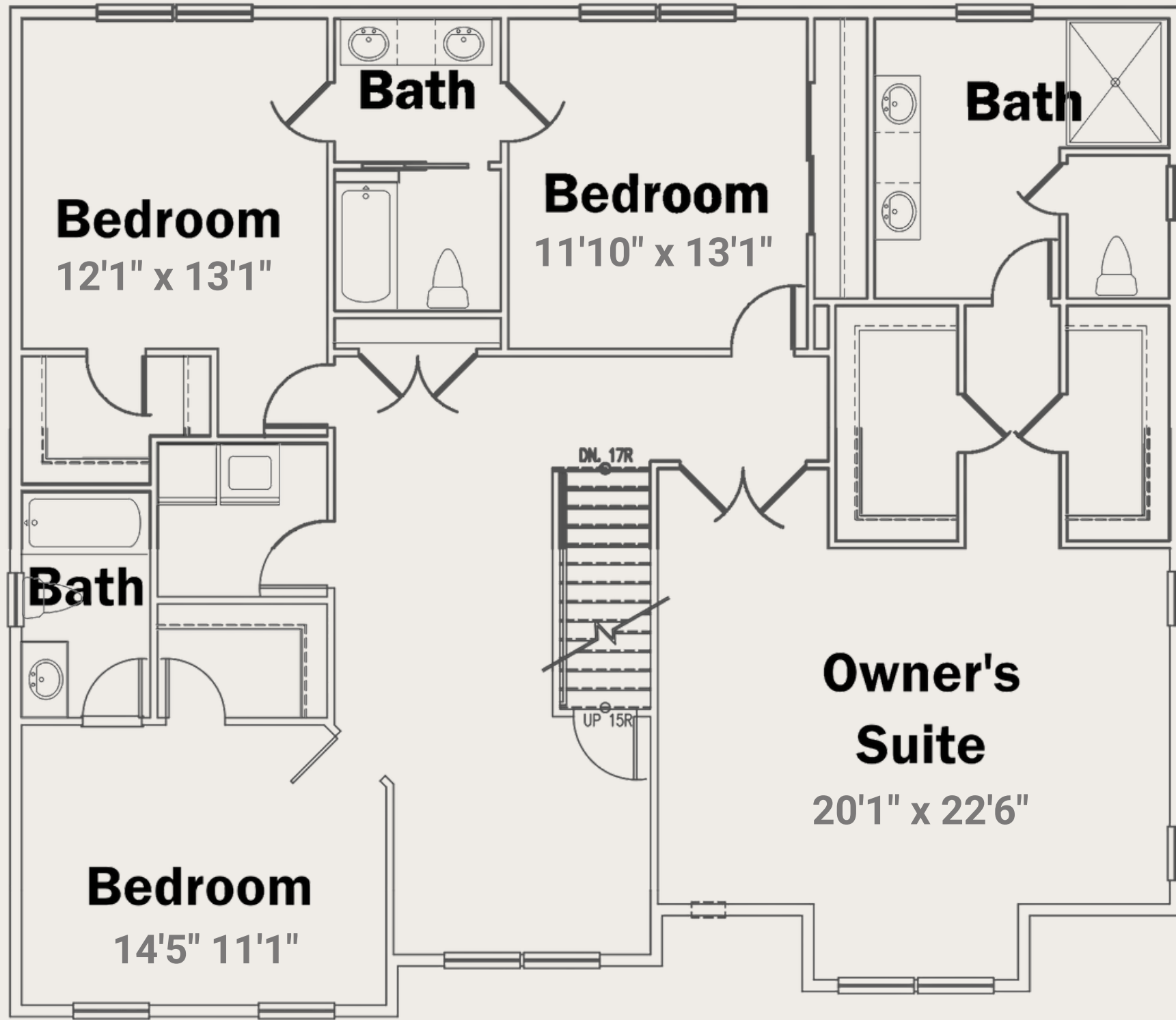
Second Floor The Princeton
